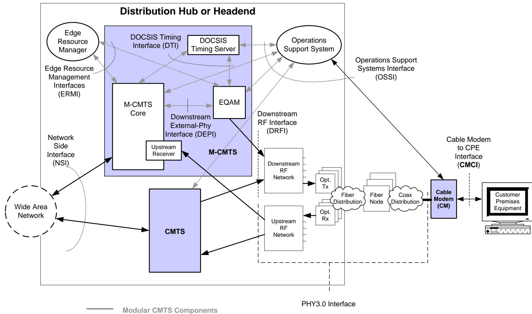
Figure 5-2 Data-Over-Cable Reference Architecture
