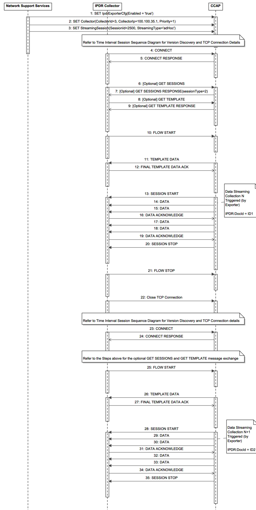
Figure 68 - IPDR/SP Streaming Telemetry Ad-hoc Session Sequence Diagram
