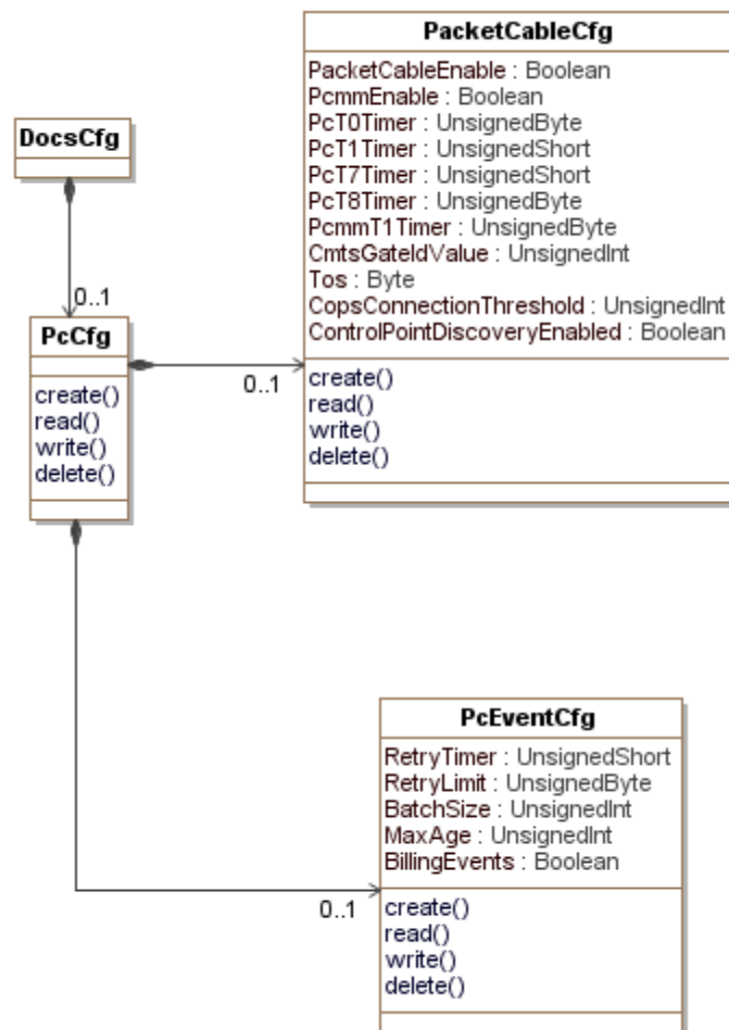
Figure 22 - PacketCable Configuration Information Model
