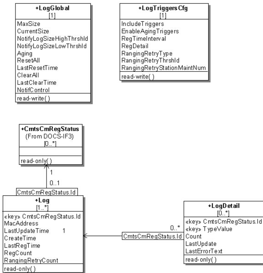
Figure 80 - Diagnostic Log Information Model
