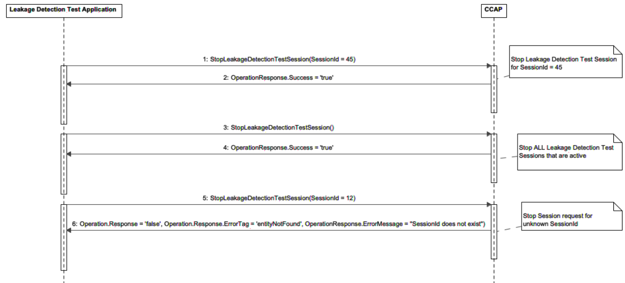
Figure 76 - Leakage Detection Test Stop Active Session
