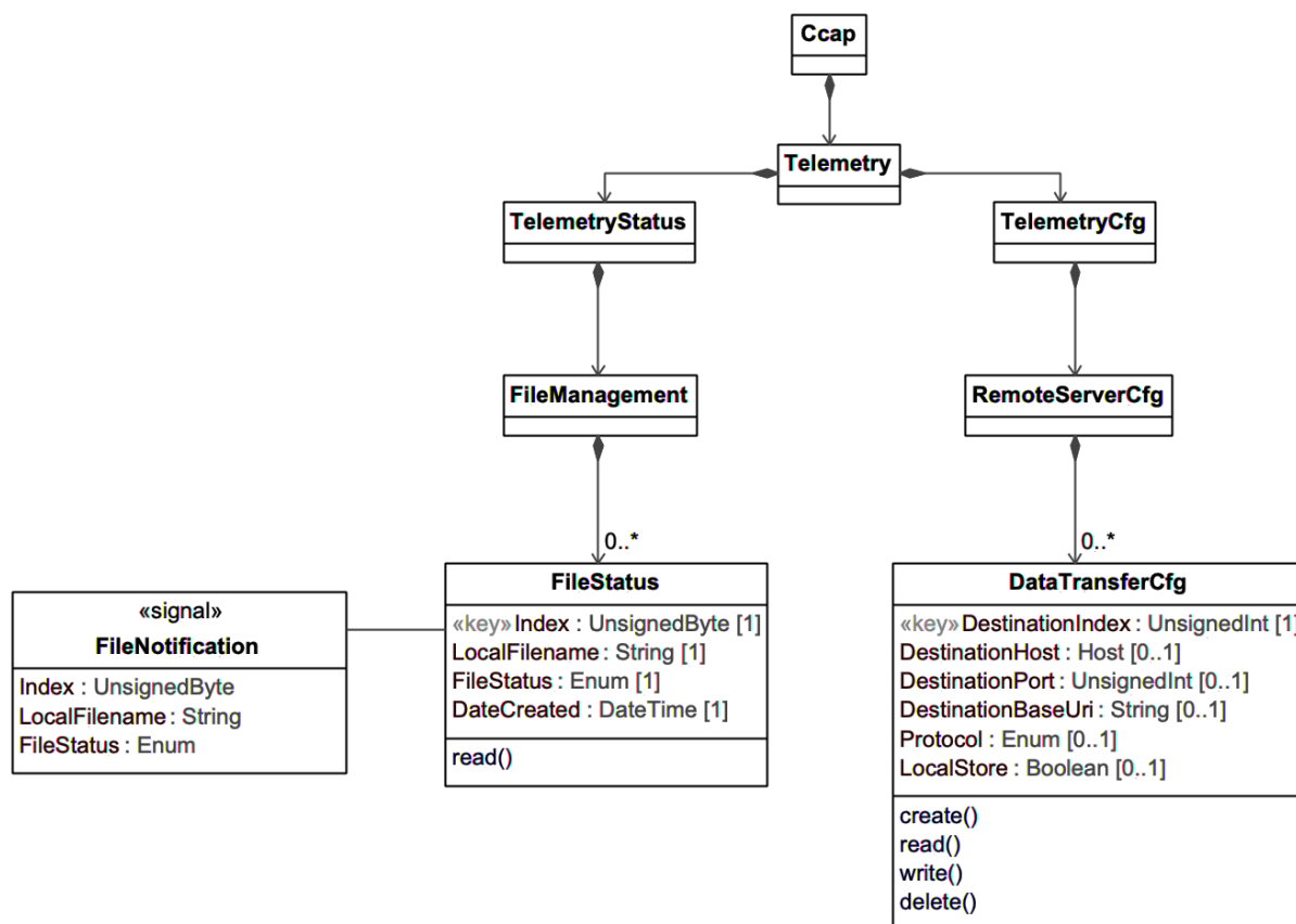
Figure 61 - Bulk File Transfer Information Model
