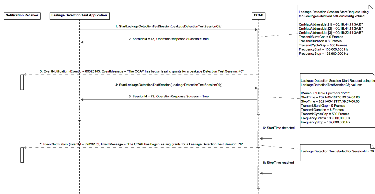
Figure 75 - Start New Leakage Detection Test Session Sequence Diagram
