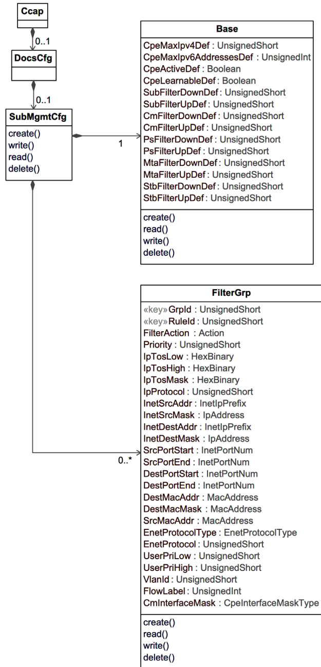
Figure 14 - DOCSIS Subscriber Management Configuration Information Model
