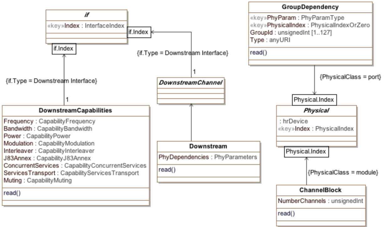
Figure 45 - DOCS-DRF-MIB Performance Management State Information Model
