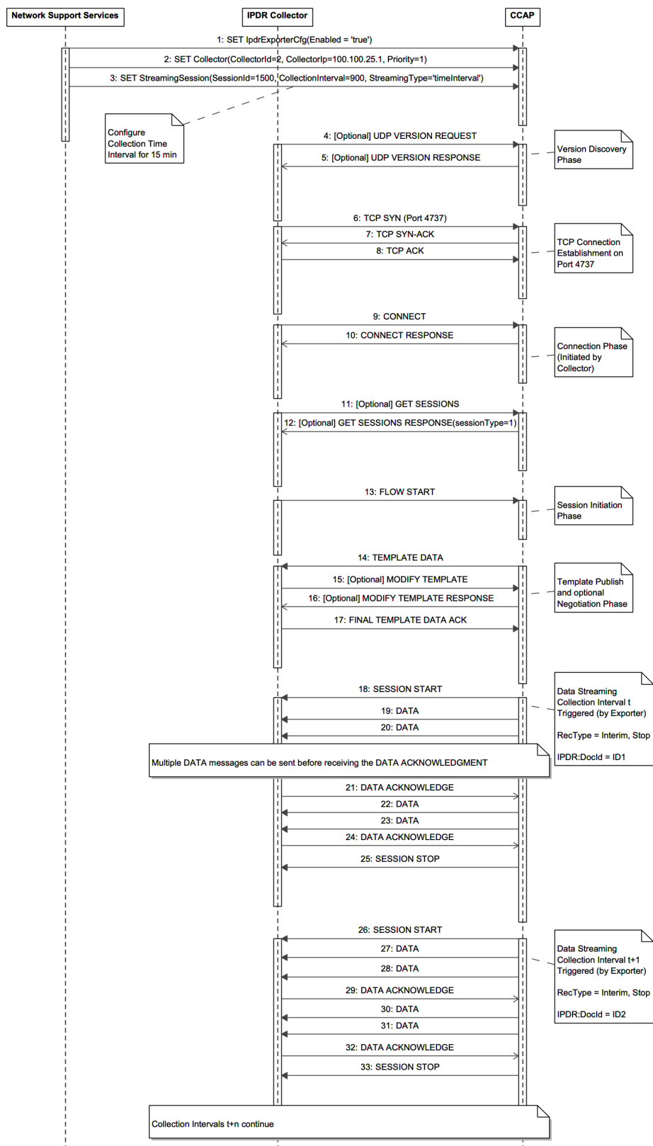
Figure 66 - IPDR/SP Streaming Telemetry Time Interval Session Sequence Diagram
