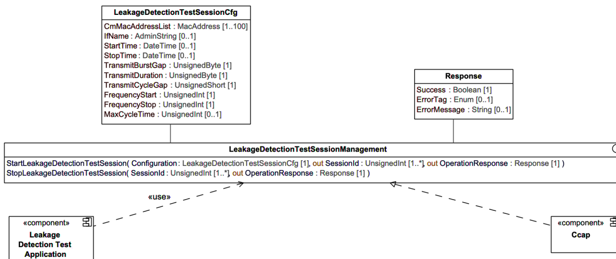
Figure 74 - DOCSIS Leakage Detection Test Component Diagram
