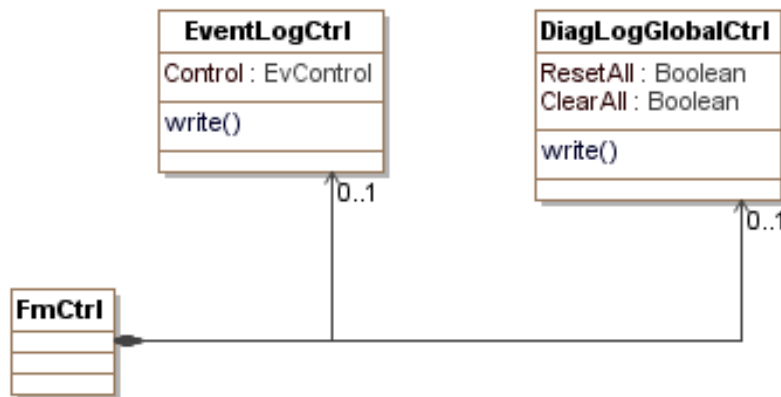
Figure 31 - Fault Management Control Information Model
