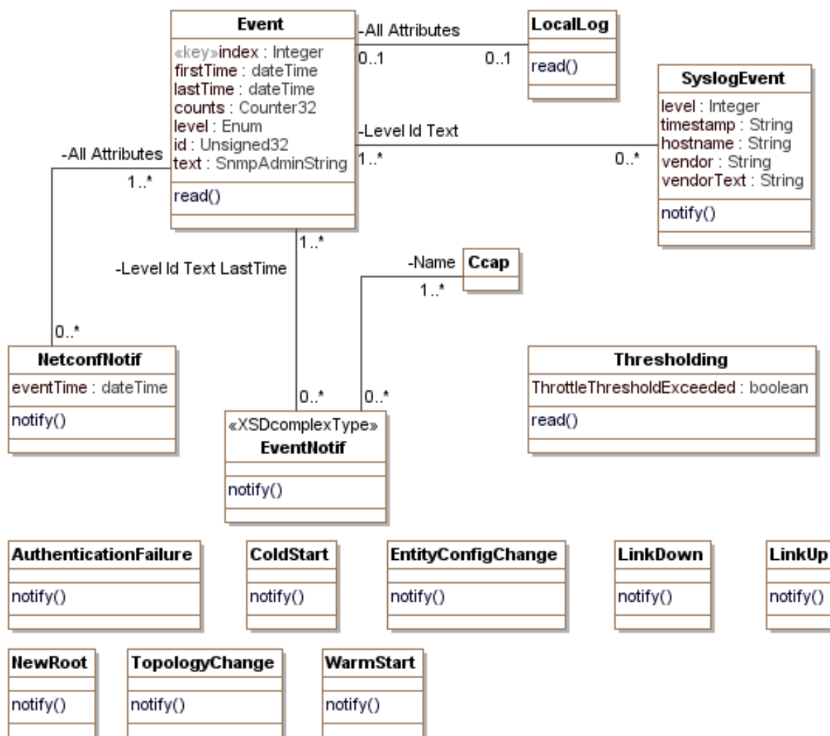
Figure 71 - CCAP Event Notification Information Model
