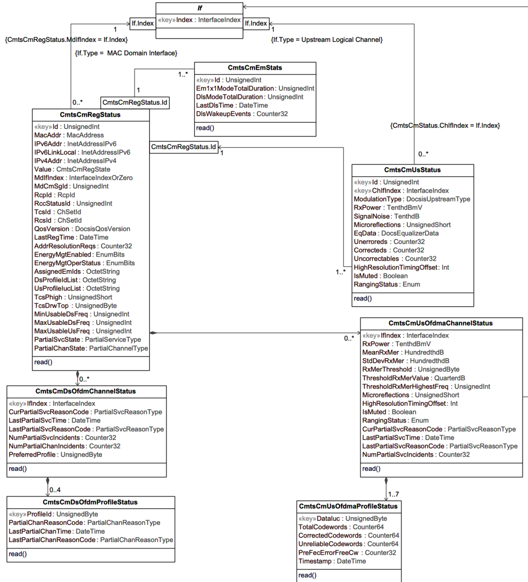
Figure 47 - CMTS CM Status Information Model
