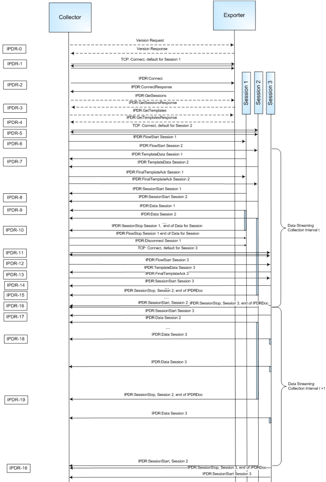
Figure 69 - Sequence Diagram for a Multisession Streaming Example
