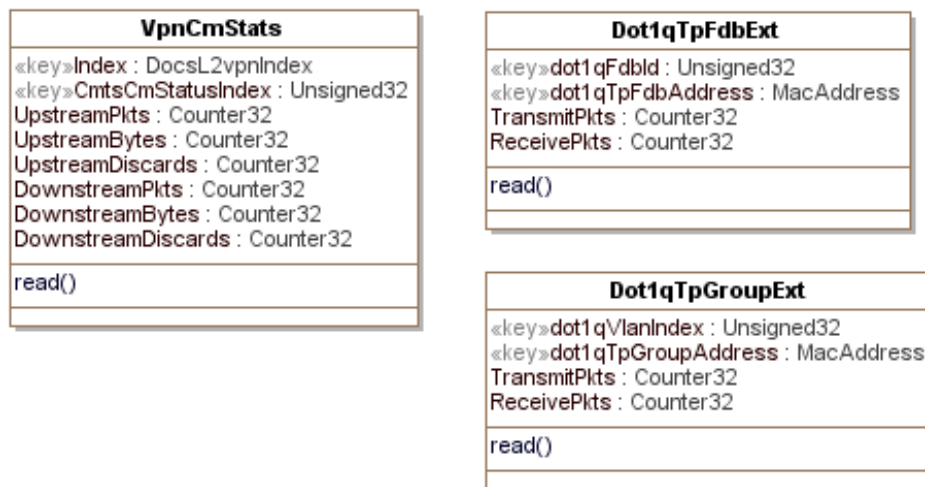
Figure 49 - DOCS-L2VPN-MIB Statistics Information Model
