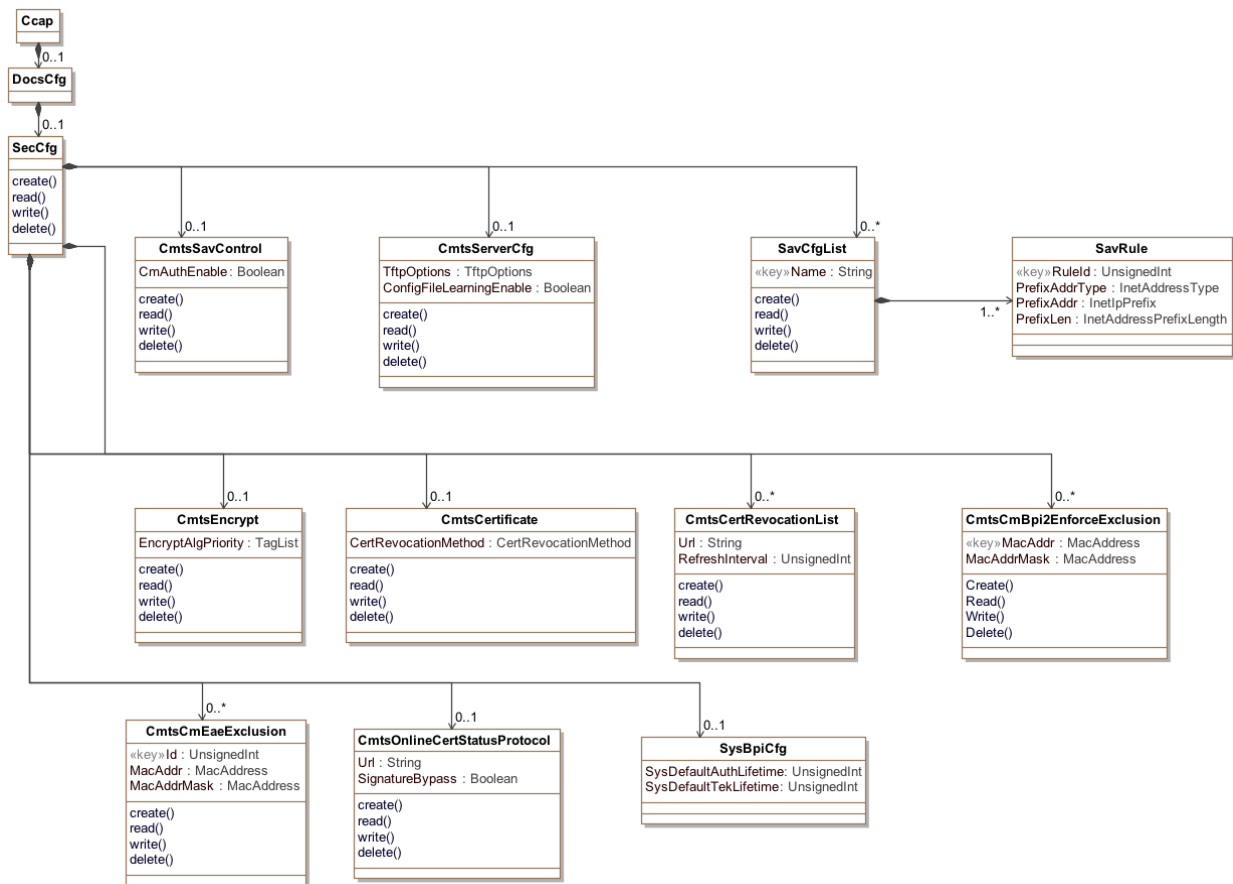
Figure 13 - DOCSIS Security Configuration Information Model
