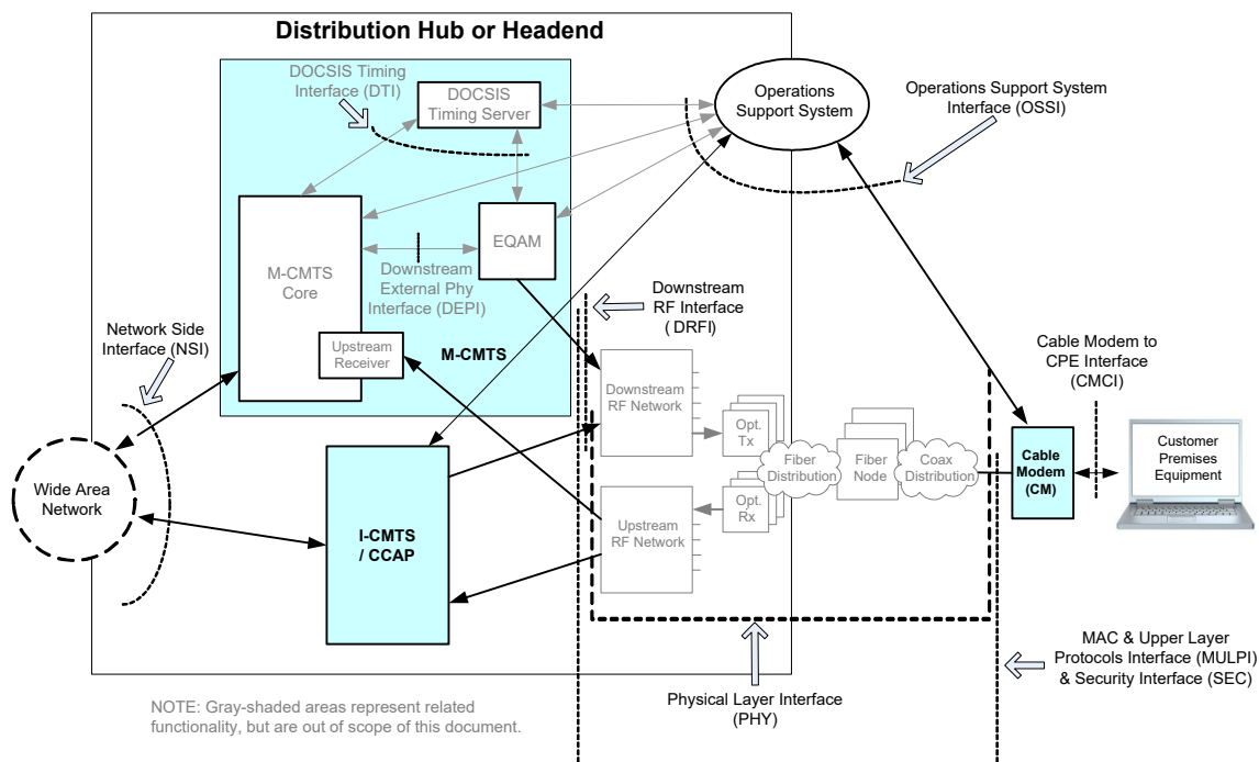
Figure 2 - Data-Over-Cable Reference Architecture
