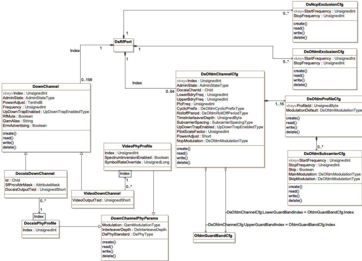
Figure 20 - Downstream DOCSIS and Video Configuration Information Model
