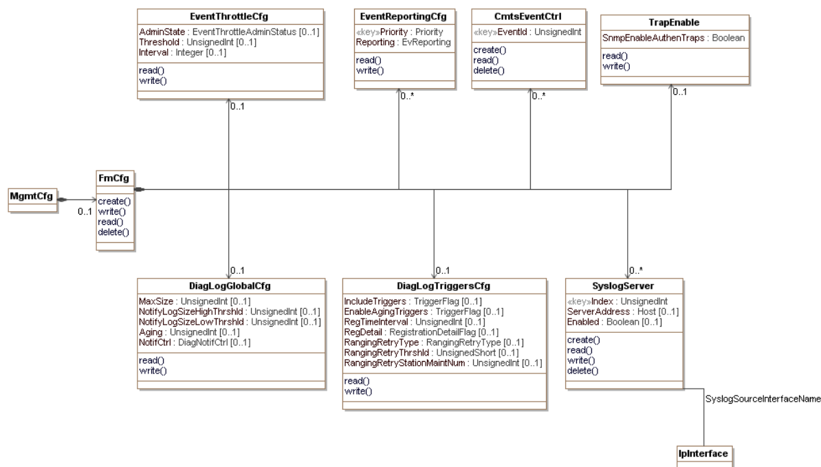
Figure 27 - Fault Management Configuration Information Model
