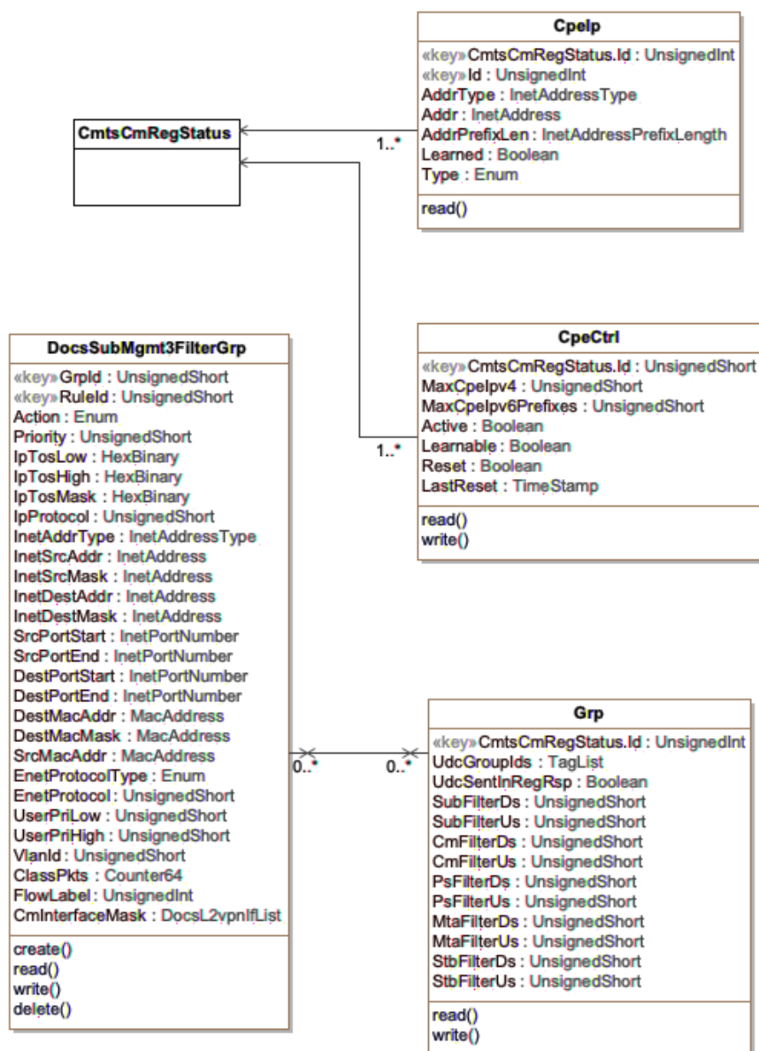
Figure 41 - DOCS-SUBMGT3-MIB Performance Management Information Model
