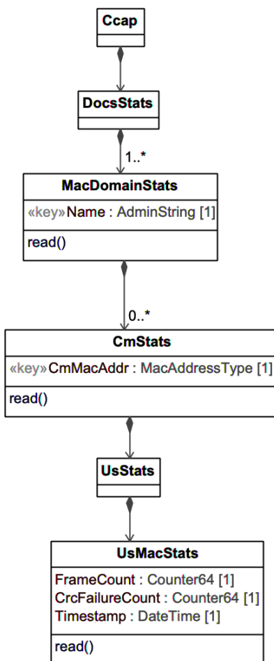
Figure 48 - MacDomainStats Information Model
