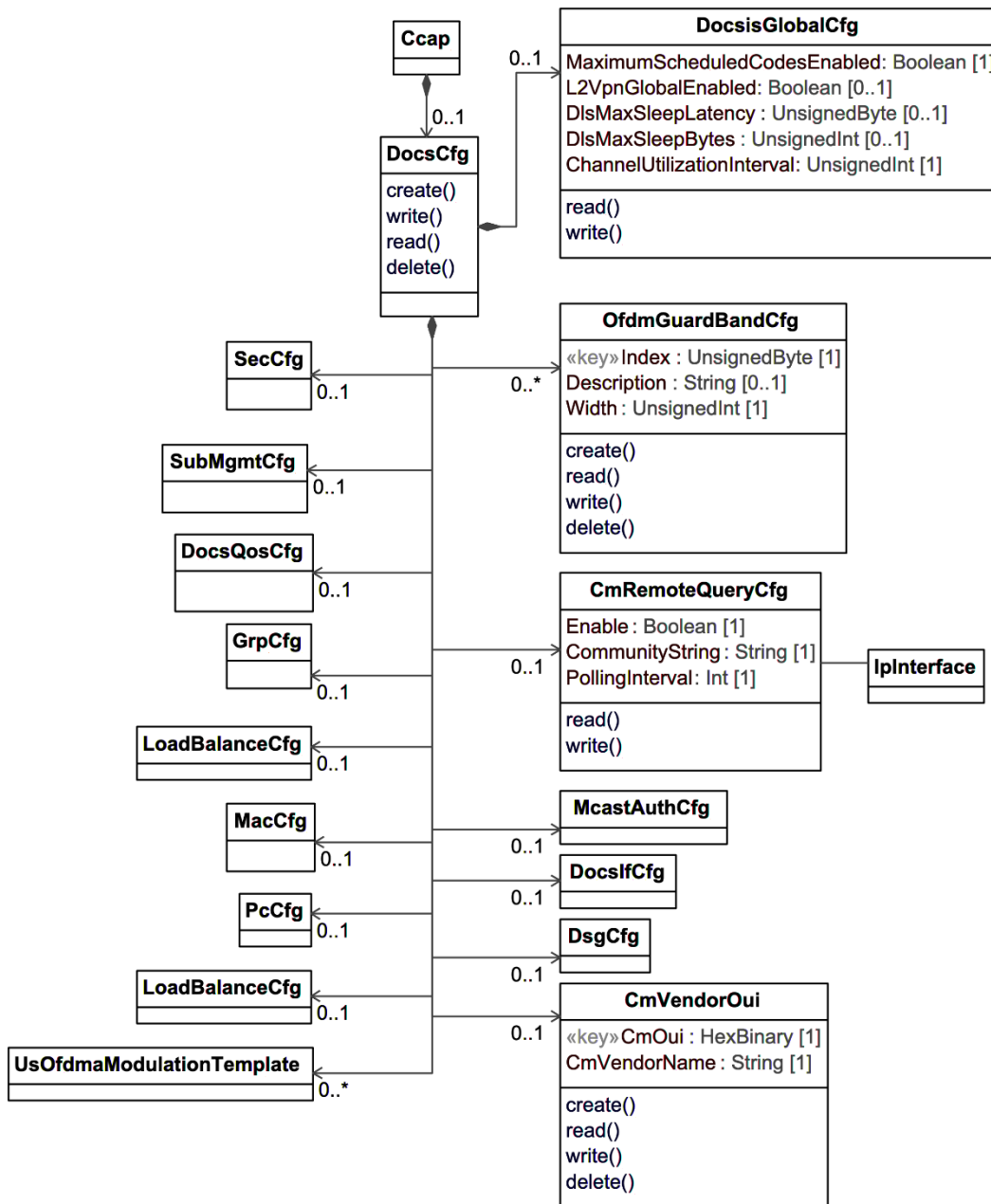
Figure 12 - DOCSIS System Configuration Information Model
