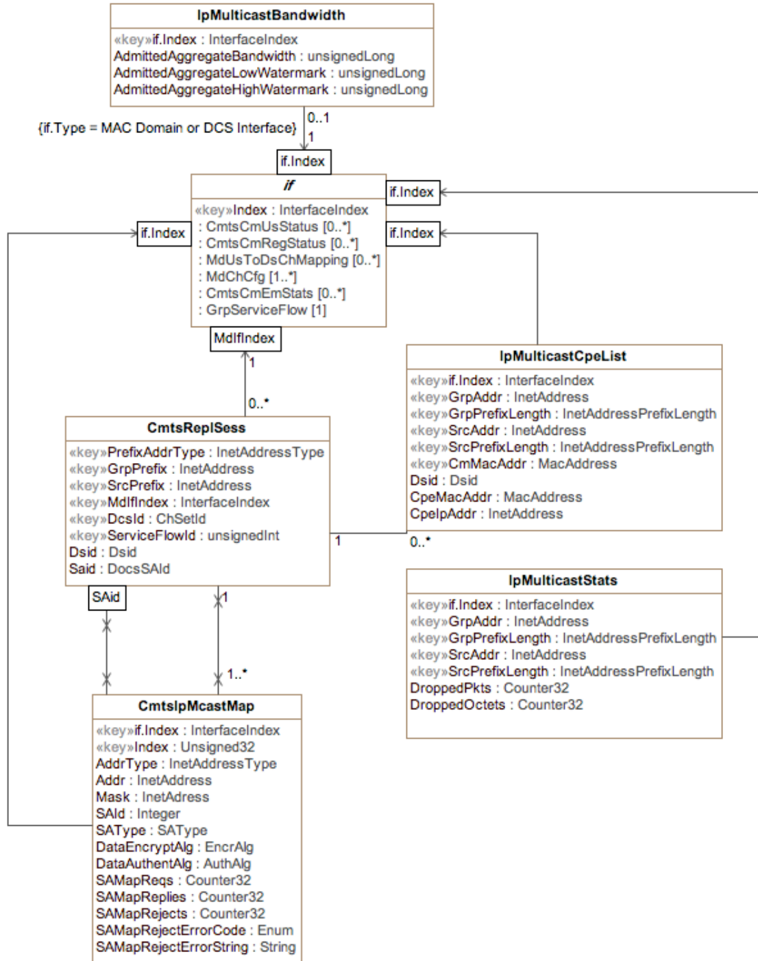
Figure 50 - DOCS-MCAST-MIB Performance Management Information Model
