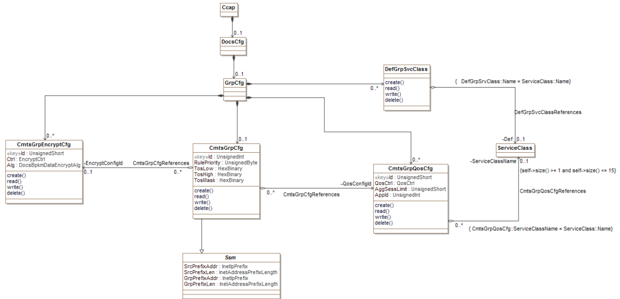
Figure 16 - DOCSIS Multicast QoS Configuration Information Model
