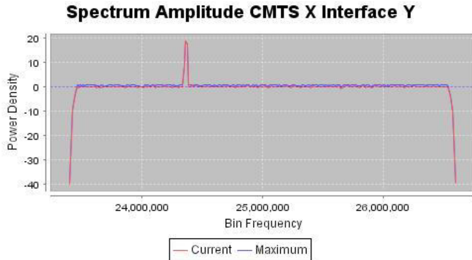
Figure 84 - Spectrum Amplitude Constructed Graph from Collected Data
