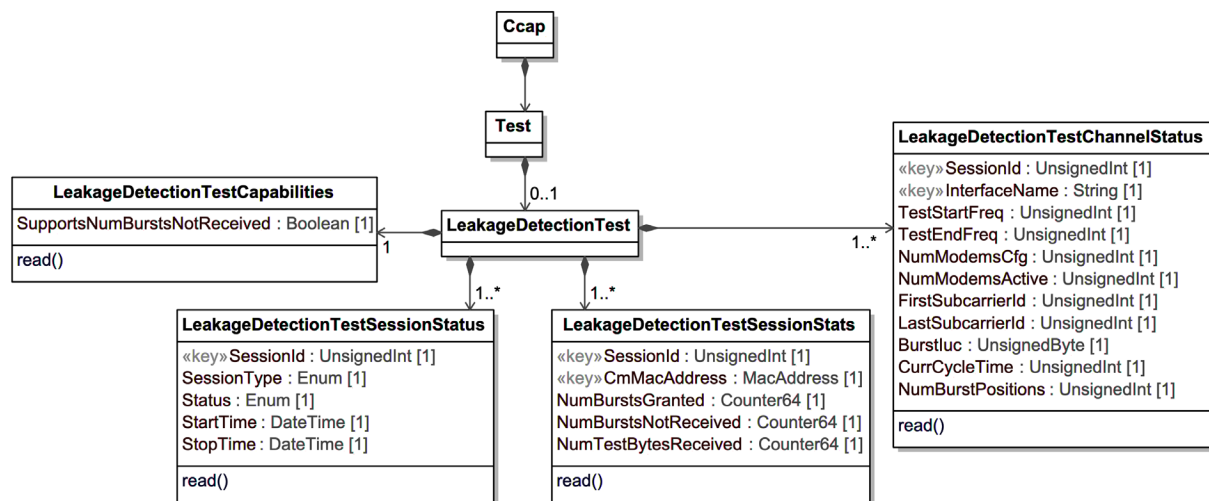
Figure 73 - Leakage Detection Test Information Model
