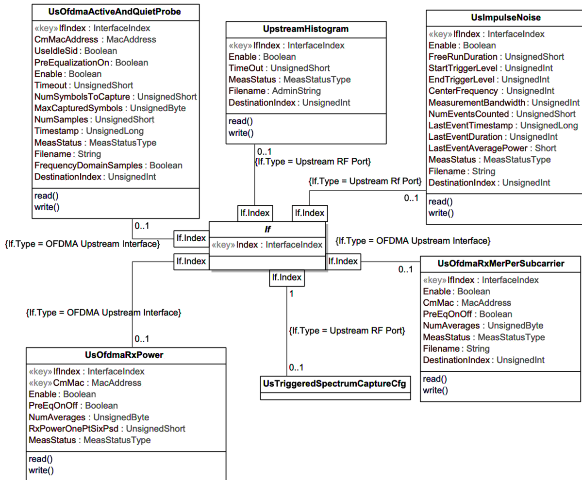
Figure 57 - PNM Upstream Information Model
