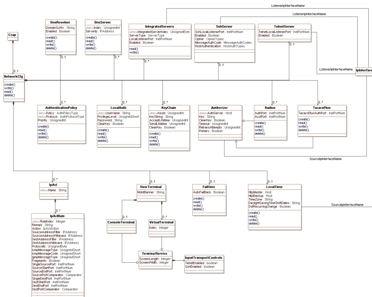
Figure 24 - CCAP Network Configuration Information Model
