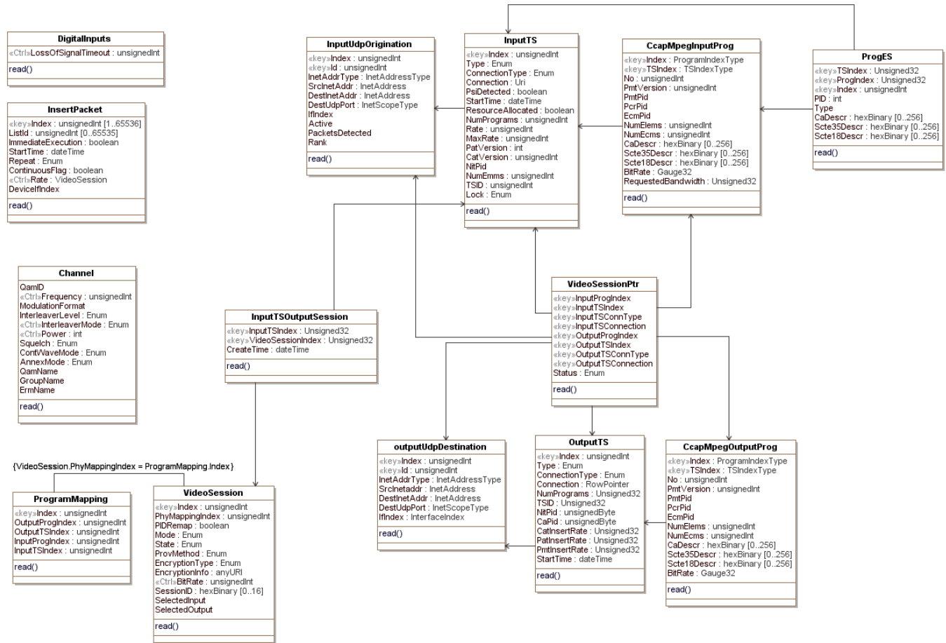
Figure 44 - SCTE-HMS-MPEG-MIB Performance Management State Information Model
