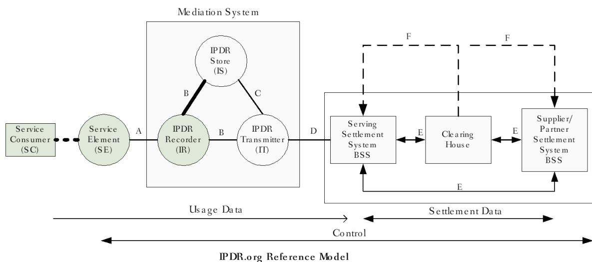
Figure 64 - Basic Network Model (IPDR/BSR)
