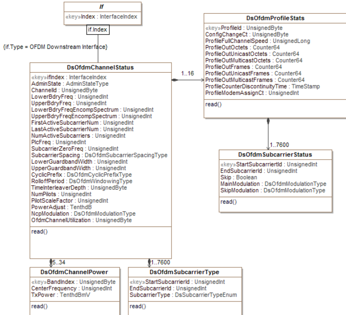
Figure 53 - Downstream OFDM Status Information Model
