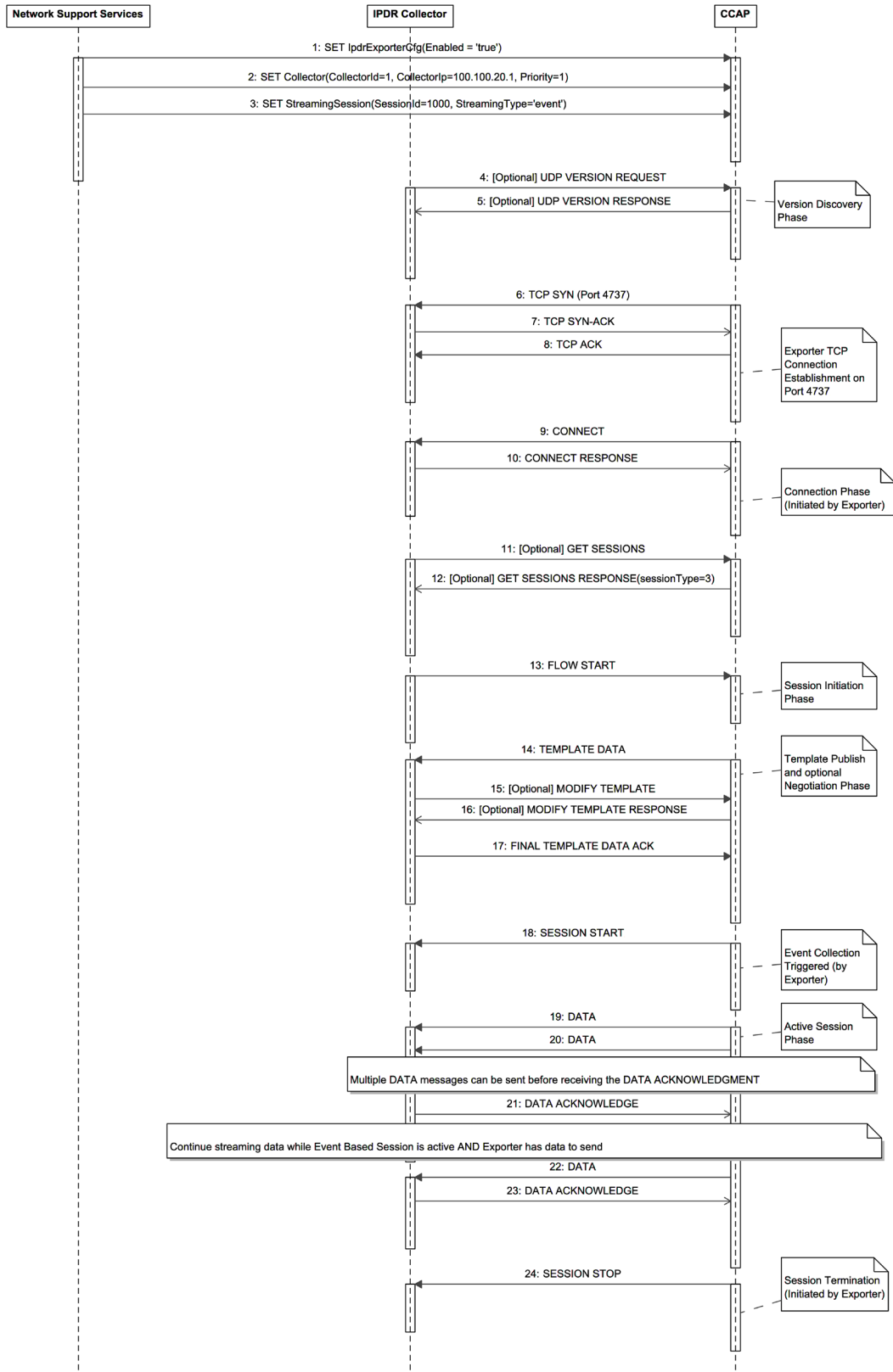
Figure 67 - IPDR/SP Streaming Telemetry Event Session Sequence Diagram
