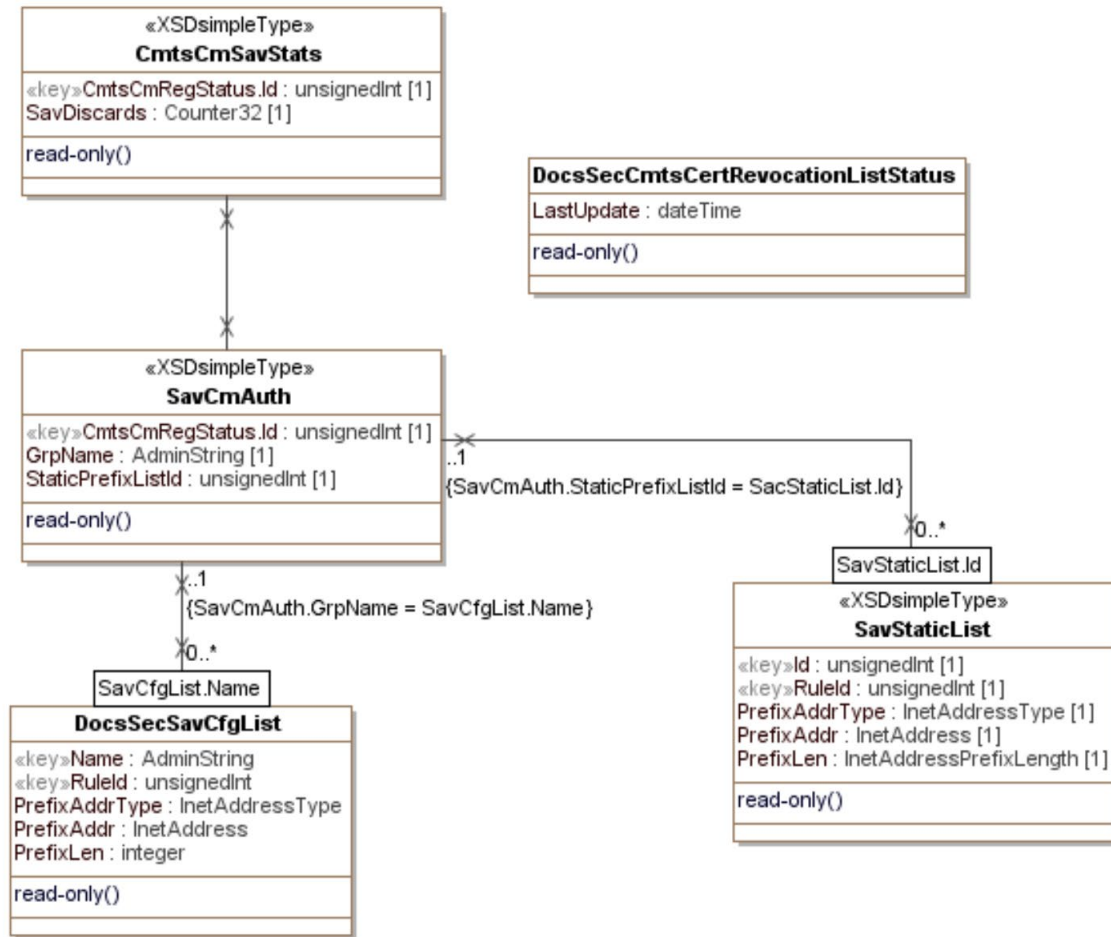
Figure 40 - DOCS-SEC-MIB Performance Management Information Model
