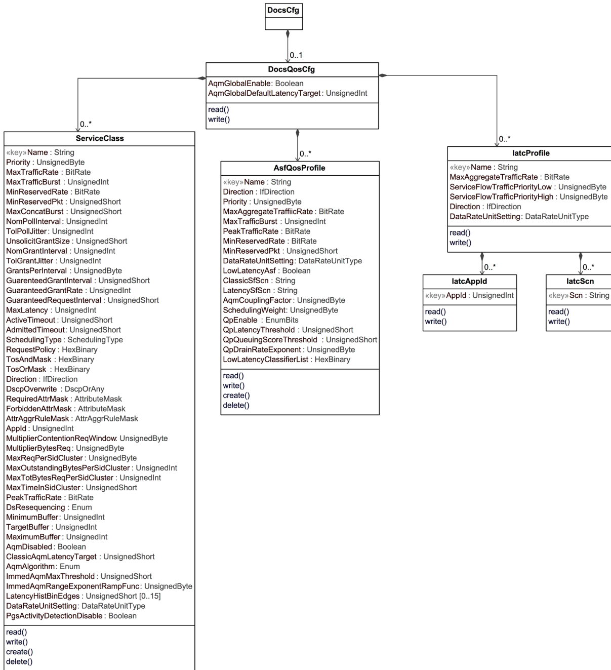
Figure 15 - DOCSIS QoS Configuration Information Model
