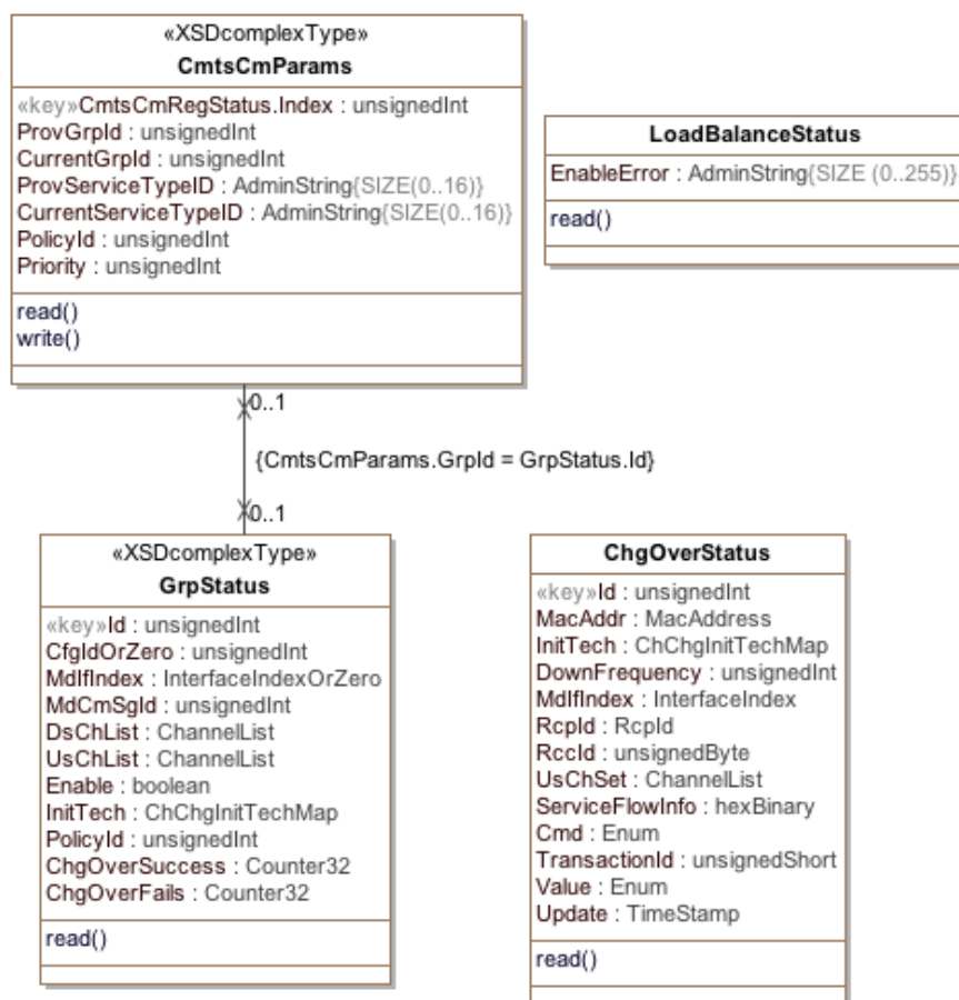
Figure 37 - DOCSIS Load Balance State Information Model
