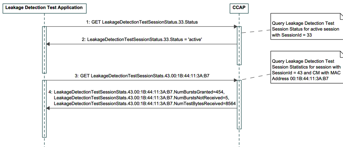
Figure 77 - Leakage Detection Test Session Status Query
