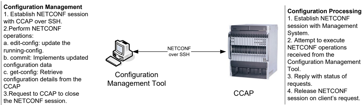
Figure 8 - CCAP NETCONF-Based Configuration Use Case
