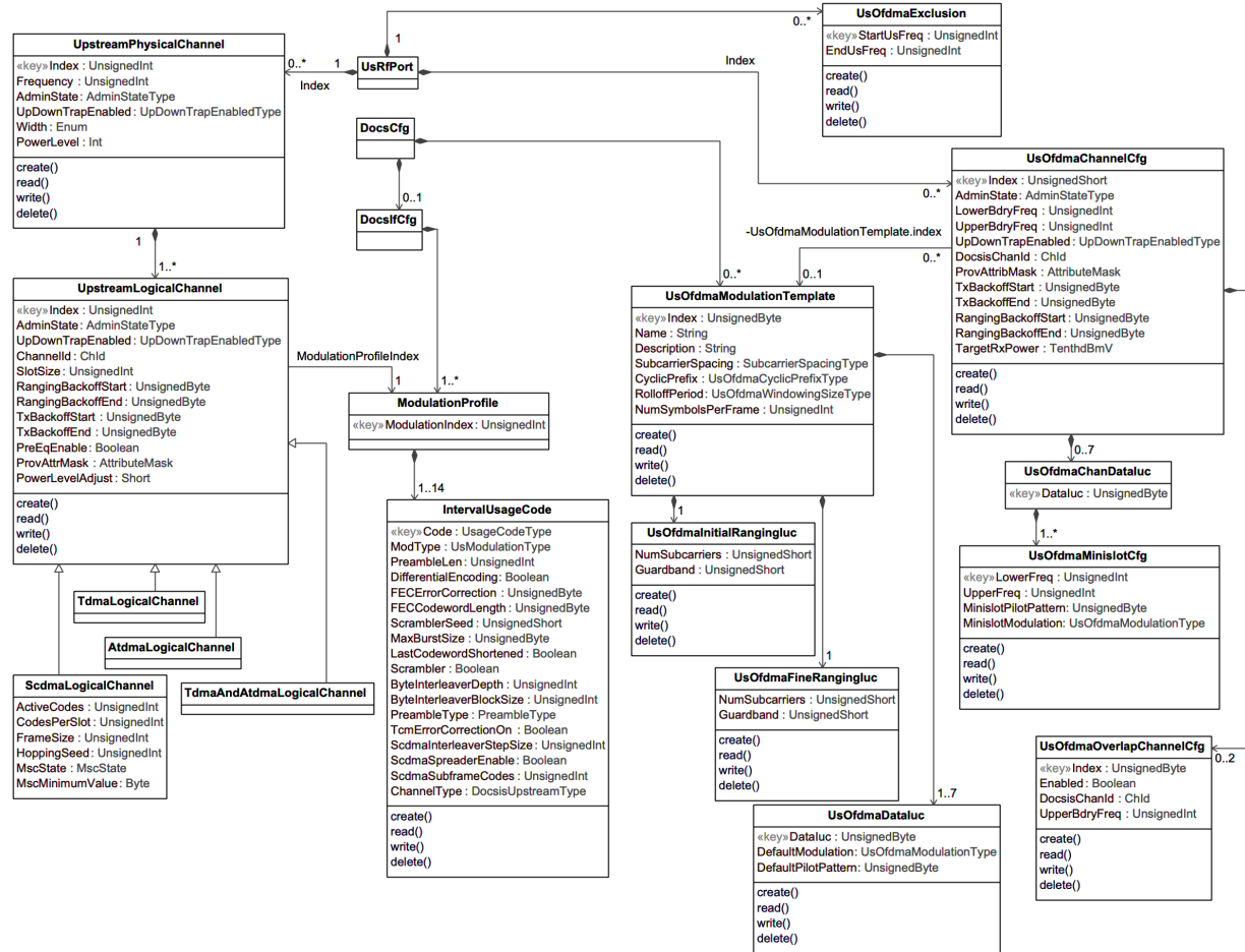
Figure 19 - DOCSIS Upstream Interface Configuration Information Model
