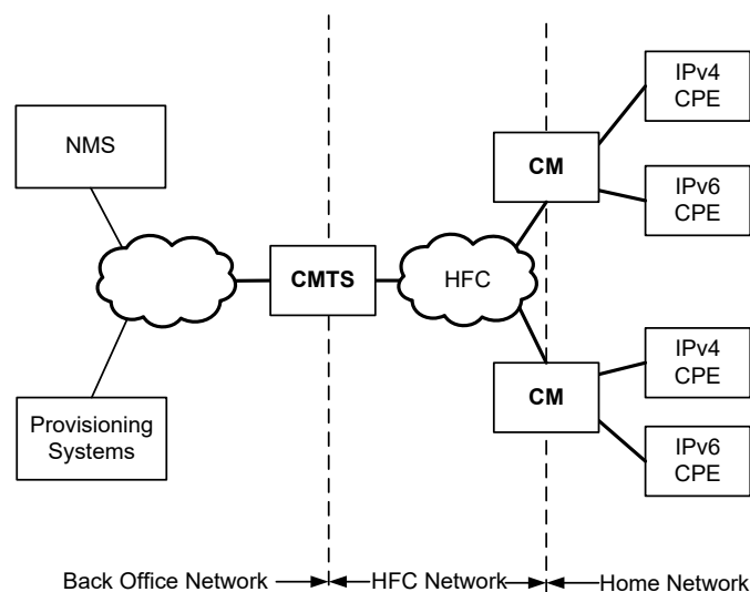
Figure 1 - The DOCSIS Network
