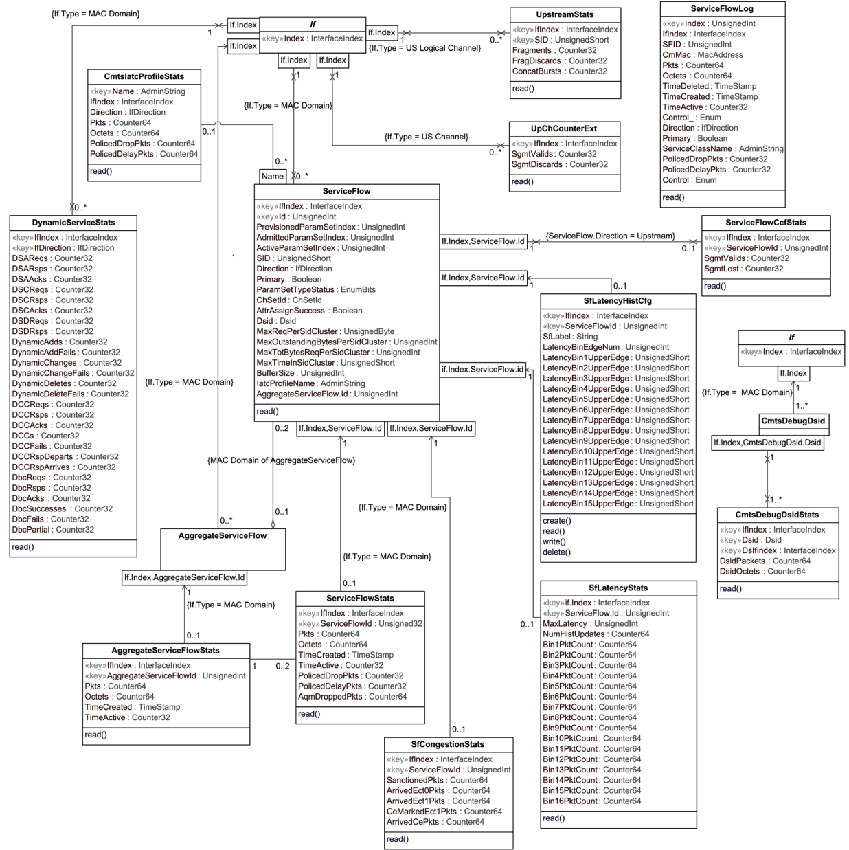
Figure 51 - DOCSIS QoS Statistical Performance Management Information Model
