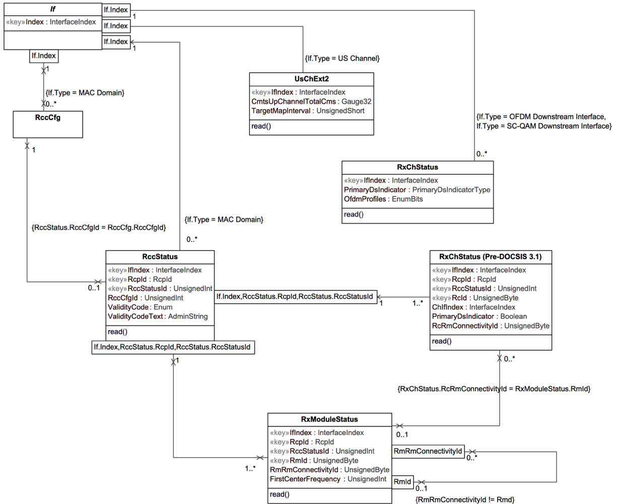
Figure 35 - Receive Channel Performance Management Information Model
