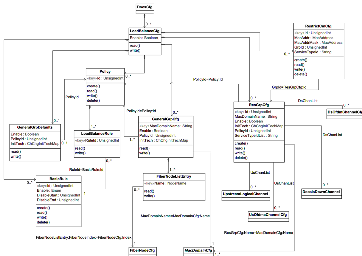
Figure 23 - Load Balance Configuration Information Model
