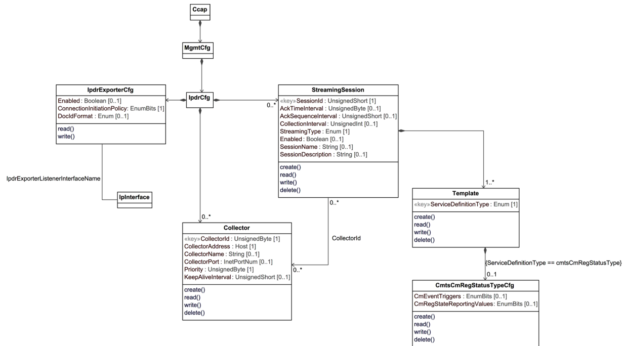
Figure 29 - IPDR Exporter Configuration Information Model
