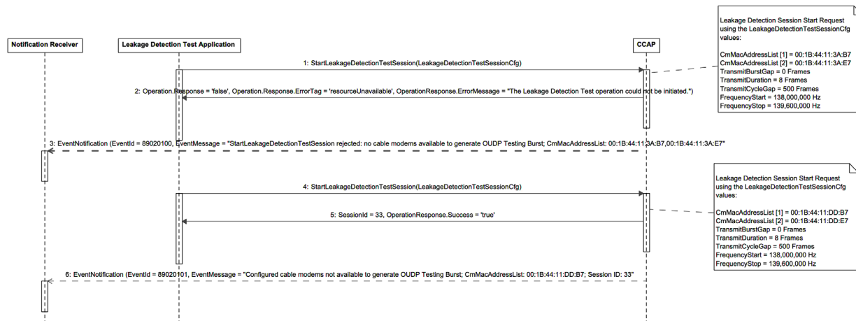
Figure 78 - Reject Start Leakage Detection Test Session Request
