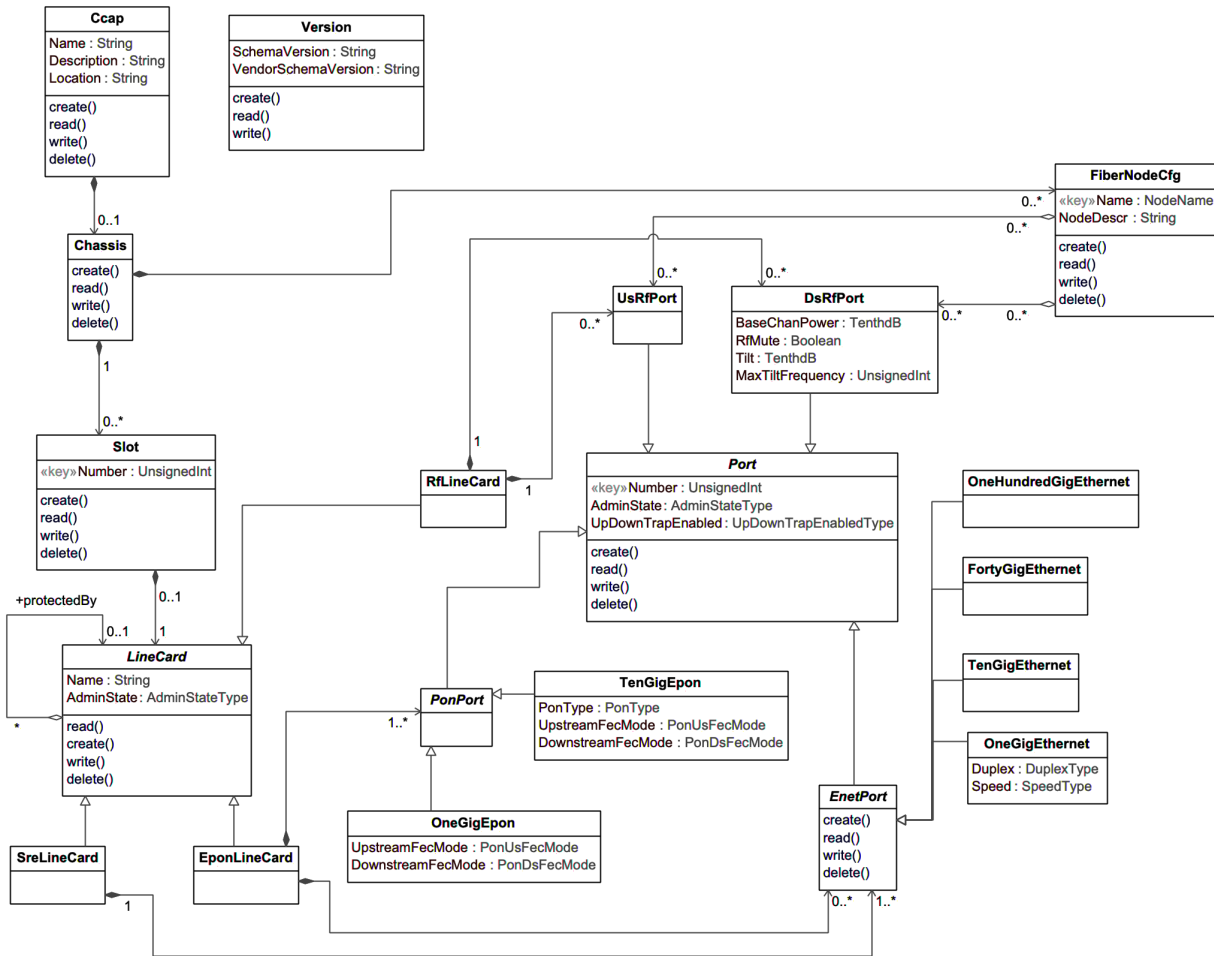
Figure 10 - CCAP Chassis Information Model
