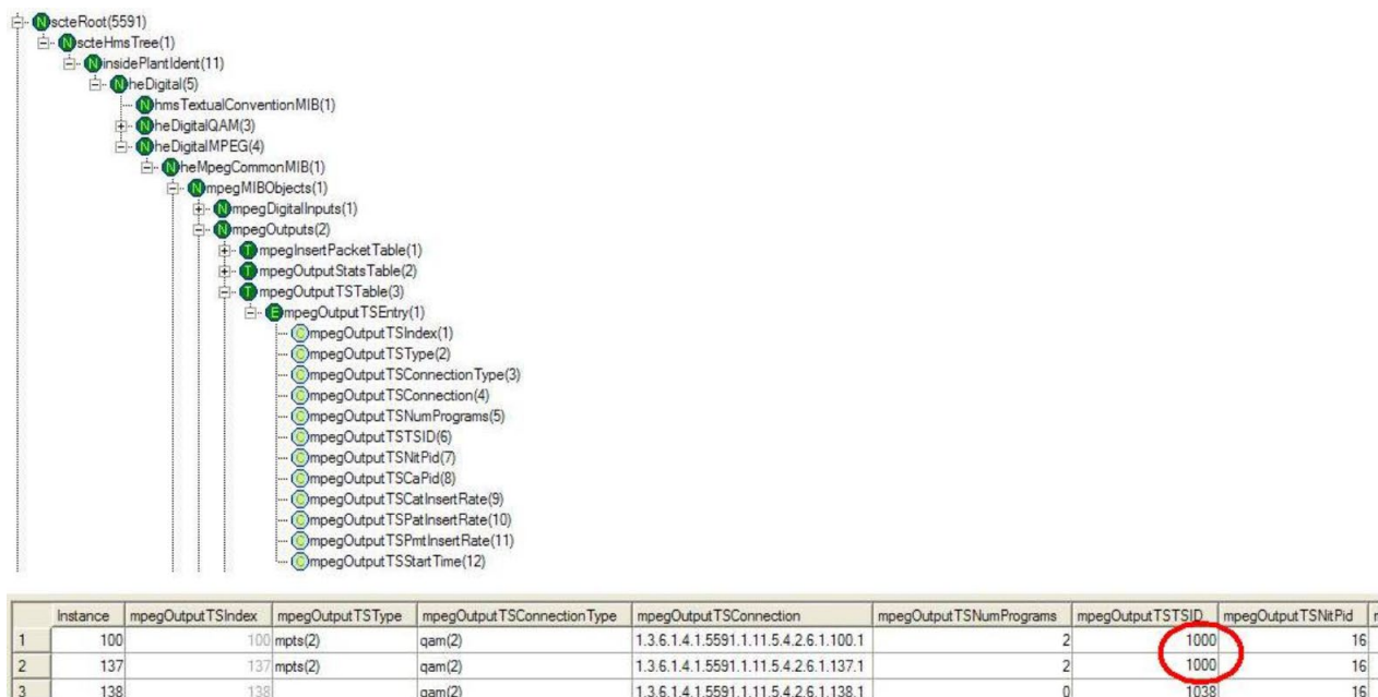
Figure 81 - Identifying a Replicated QAM by Looking at mpegOutputTSTSID
