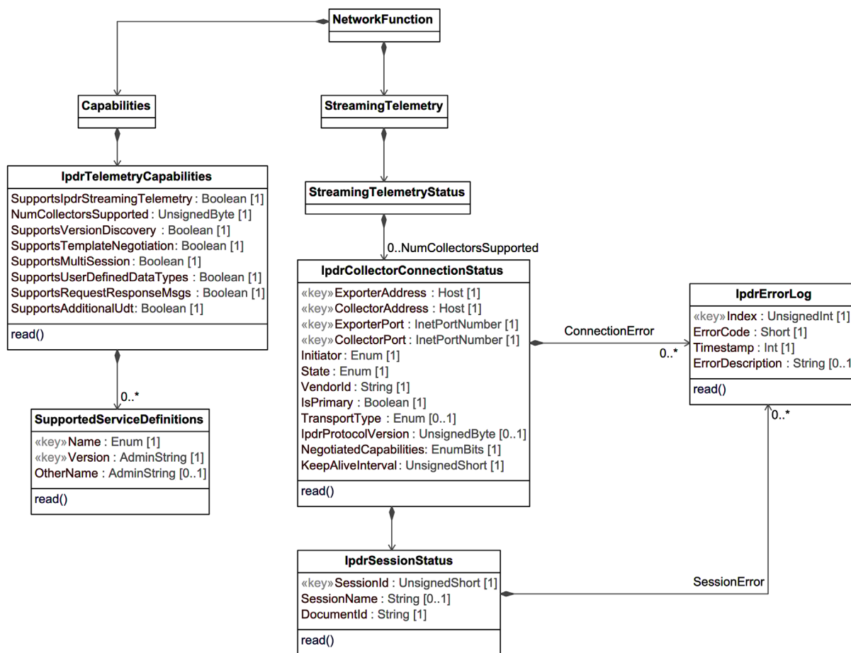
Figure 63 - IPDR Streaming Telemetry Status Information Model
