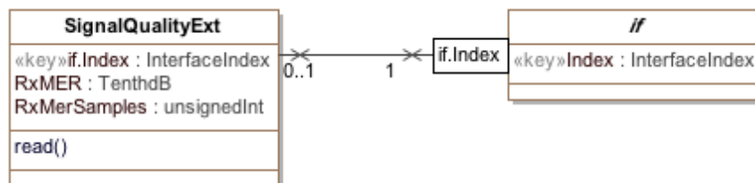
Figure 54 - DOCS-IF3-MIB Statistical Performance Management Information Model
