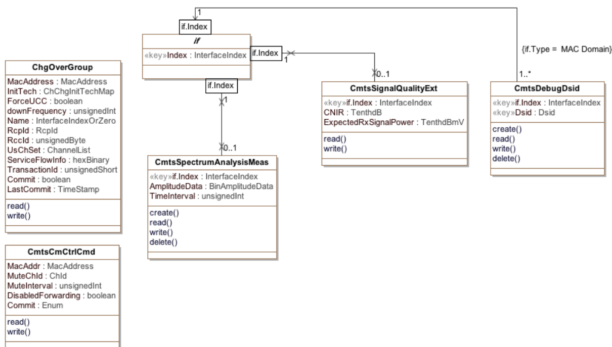
Figure 32 - Performance Management Control and Monitoring Information Model
