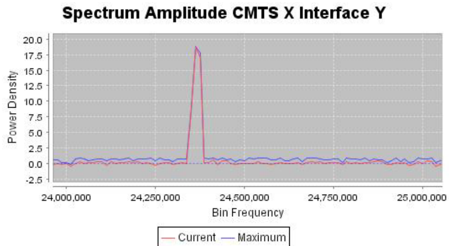
Figure 85 - Spectrum Amplitude Detail Graph from Collected Data
