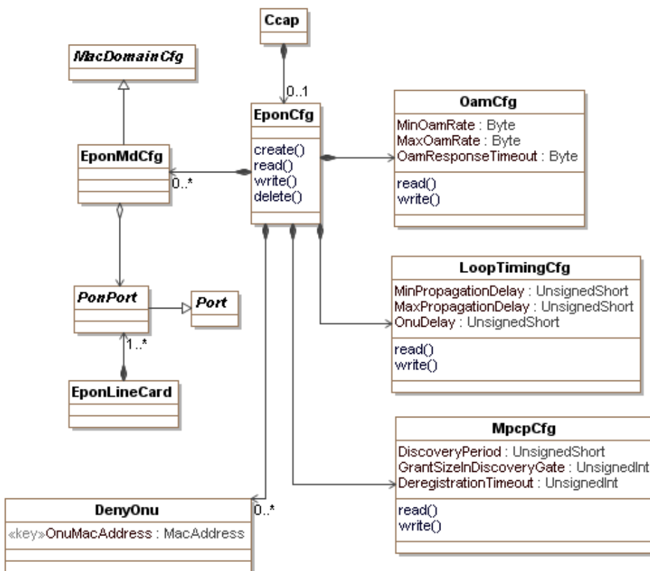
Figure 30 - EPON Configuration Information Model
