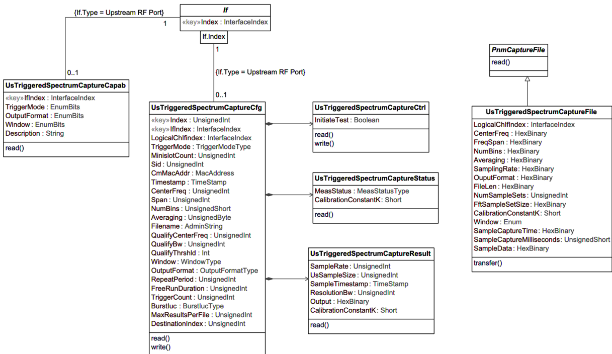
Figure 58 - Upstream Triggered Spectrum Capture Information Model
