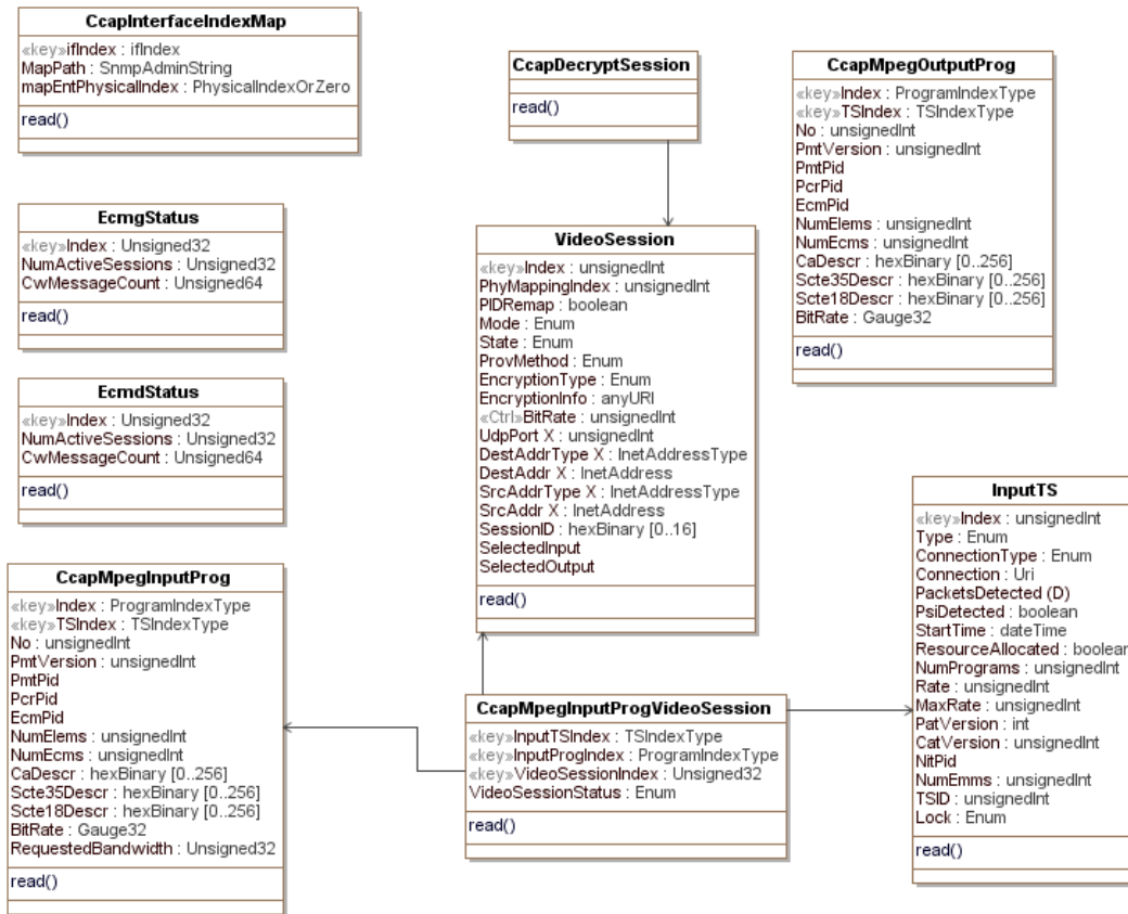
Figure 43 - CCAP-MIB Performance Management Information Model
