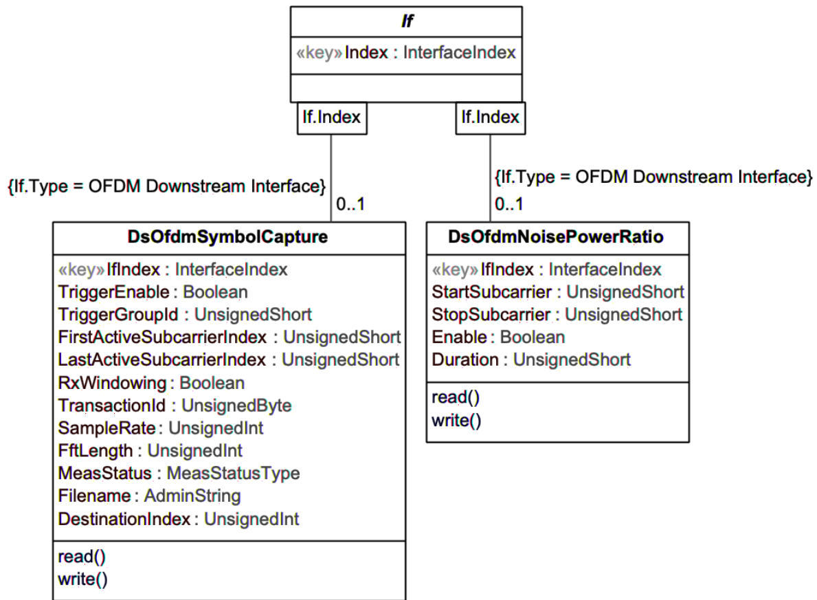
Figure 56 - PNM Downstream Information Model
