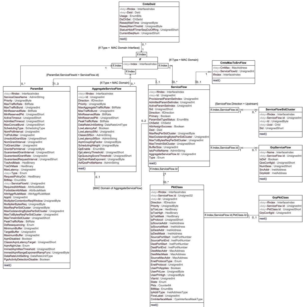
Figure 39 - DOCSIS QoS State Performance Management Information Model
