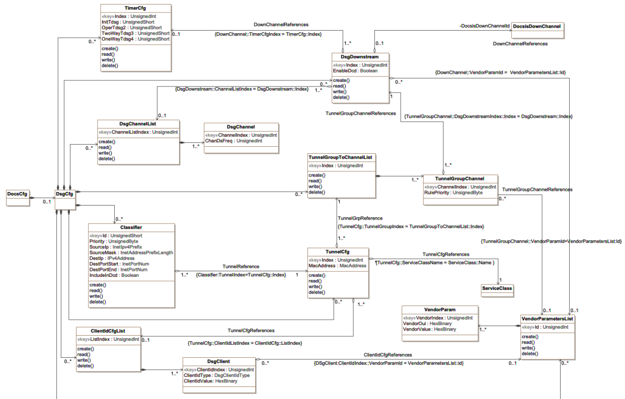
Figure 21 - DSG Configuration Information Model
