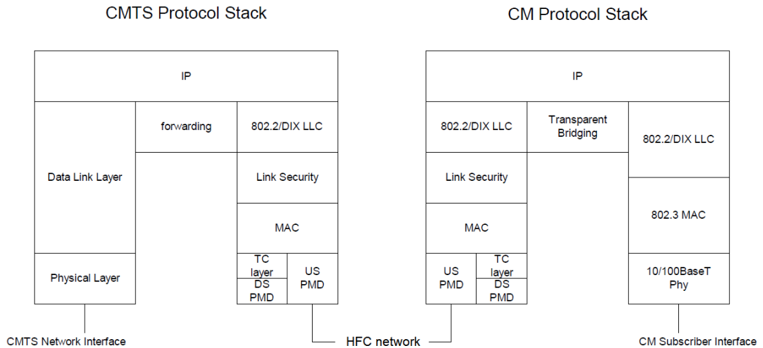
Figure 2.2.: DOCSIS-Stack of CMTS and CM [3]
