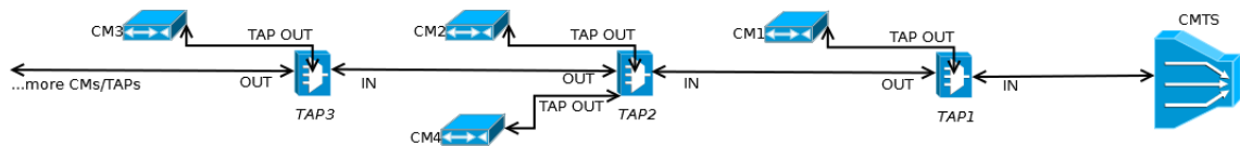
Figure 4.2.: Simplified cable plant example
